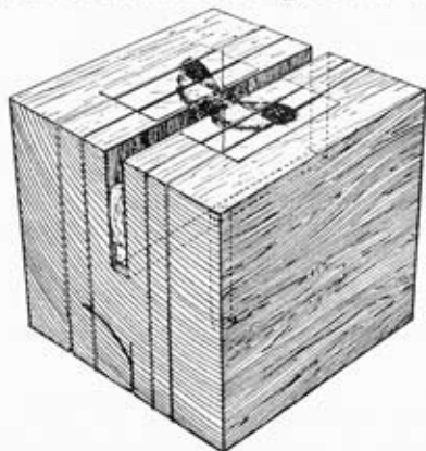
FIGURE 14.—Construction and use of the spreading block for small insects.
